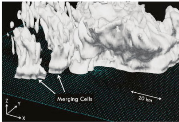
Simulated cell merger. 3-D image of the simulation as seen from southeast of the parent storm 30 minutes before peak intensity. The merging cells are noted. White shading is a 30-dBZ isosurface and blue arrows are surface wind vectors. (VAN LEER, JEWETT, AND WILHELMSON)
