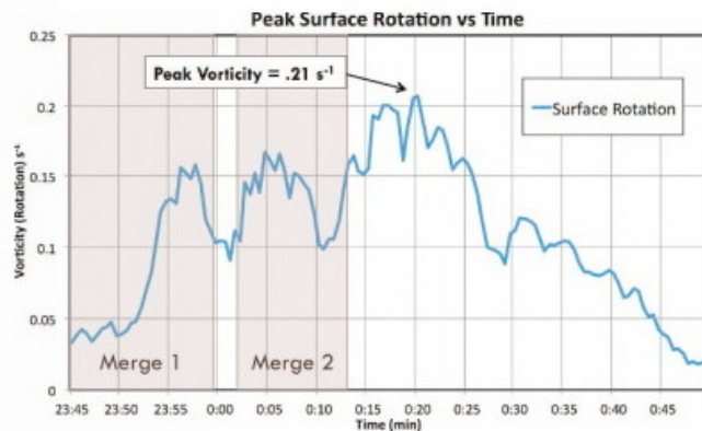
Rapid intensification. Rotation (surface vorticity, s^{-1} ) response vs. time (UTC, hour:minutes) associated with two cell mergers in the simulation. The rotation in this simulation is on the same scale as a tornado-strength vortex. (VAN LEER, JEWETT, AND WILHELMSON)
