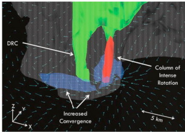
Powerful rotation. 3-D image as seen from southeast of the surface circulation (blue vectors) during the time of peak intensity. Red is a 0.1 \text{ s}^{-1} vorticity isosurface, blue is a 0.025 \text{ s}^{-1} convergence isosurface, and reflectivity is gray (30 dBZ) and green (55 dBZ). (VAN LEER, JEWETT, AND WILHELMSON)
