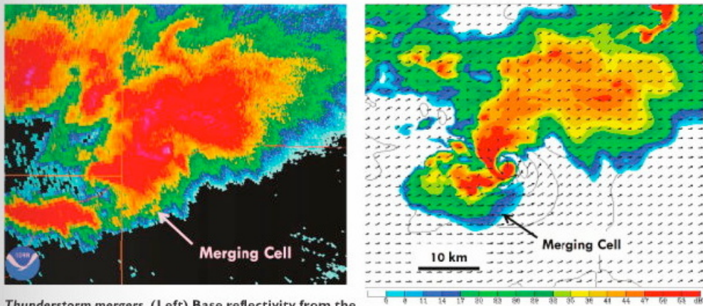
Thunderstorm mergers. (Left) Base reflectivity from the KSGF WSR-88D radar at 2243 UTC on 22 May 2011. A weaker cell is merging with the primary storm along the northwest Arkansas-southwest Missouri border. (Right) Surface wind and reflectivity at 2 km AGL in the same area, from the WRF simulation. (VAN LEER, JEWETT, AND WILHELMSON)
